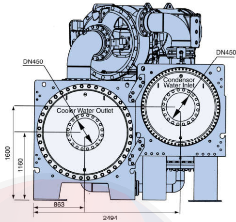
Compressor End View
