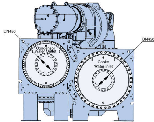
Motor End View
