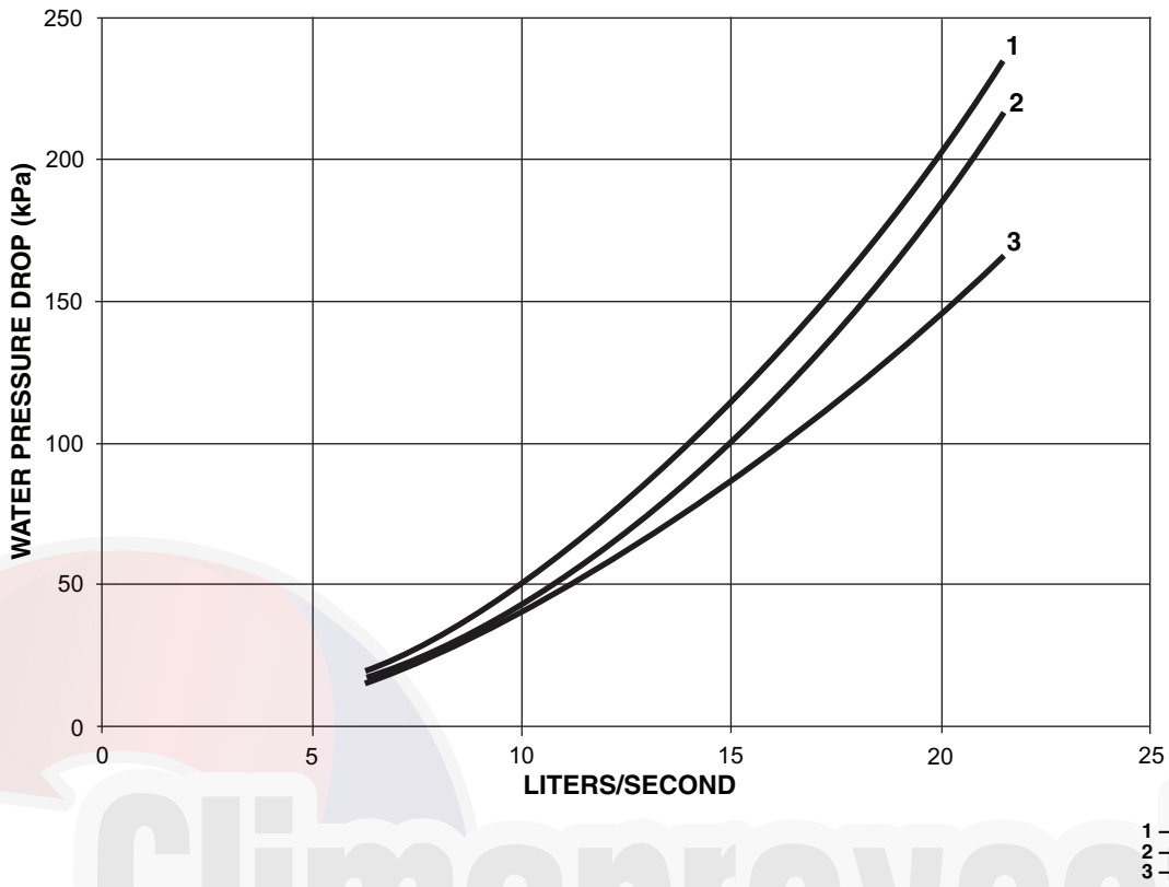
UNIT PRESSURE DROP — NO HYDRONIC PACKAGE — 30RAP070-090 (SI)
