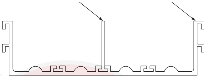
Fig. 180 — 2-in. Track Assembly (4-in. Track)
