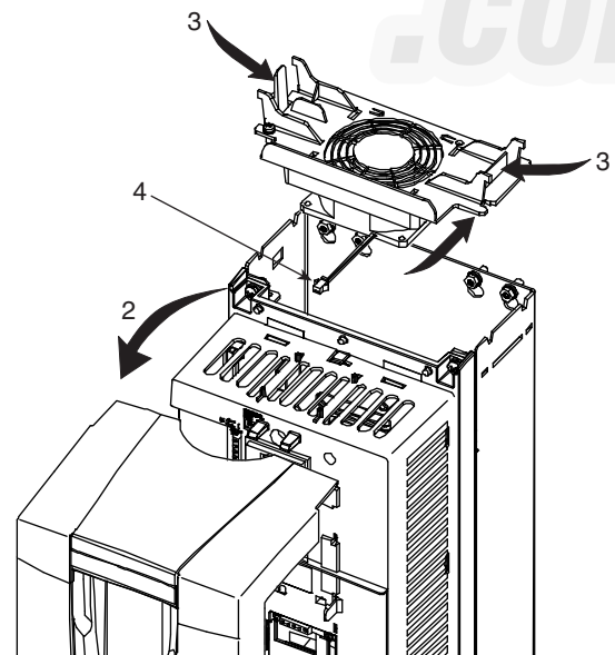
Fig. 191 — Main Fan Replacement (Frame Sizes R1 - R4)
