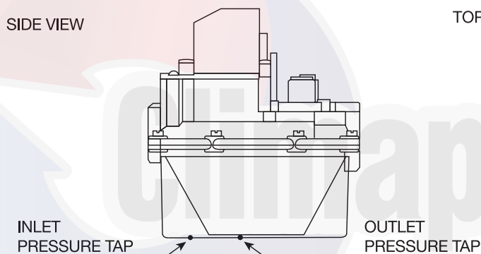
Fig. 144 — Honeywell V8944 Gas Valve
