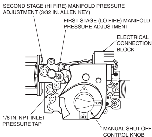
Fig. 143 — 2-Stage Gas Valve
