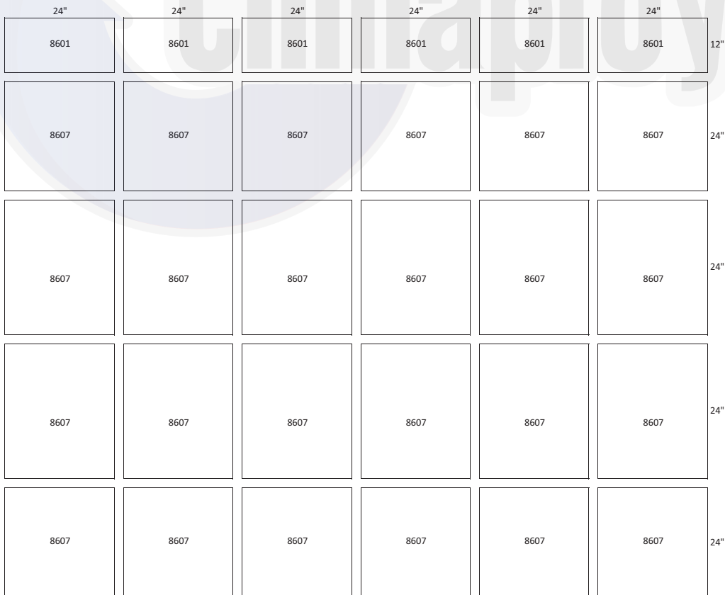
Fig. 189 — HEPA Filter Arrangement (cont)
