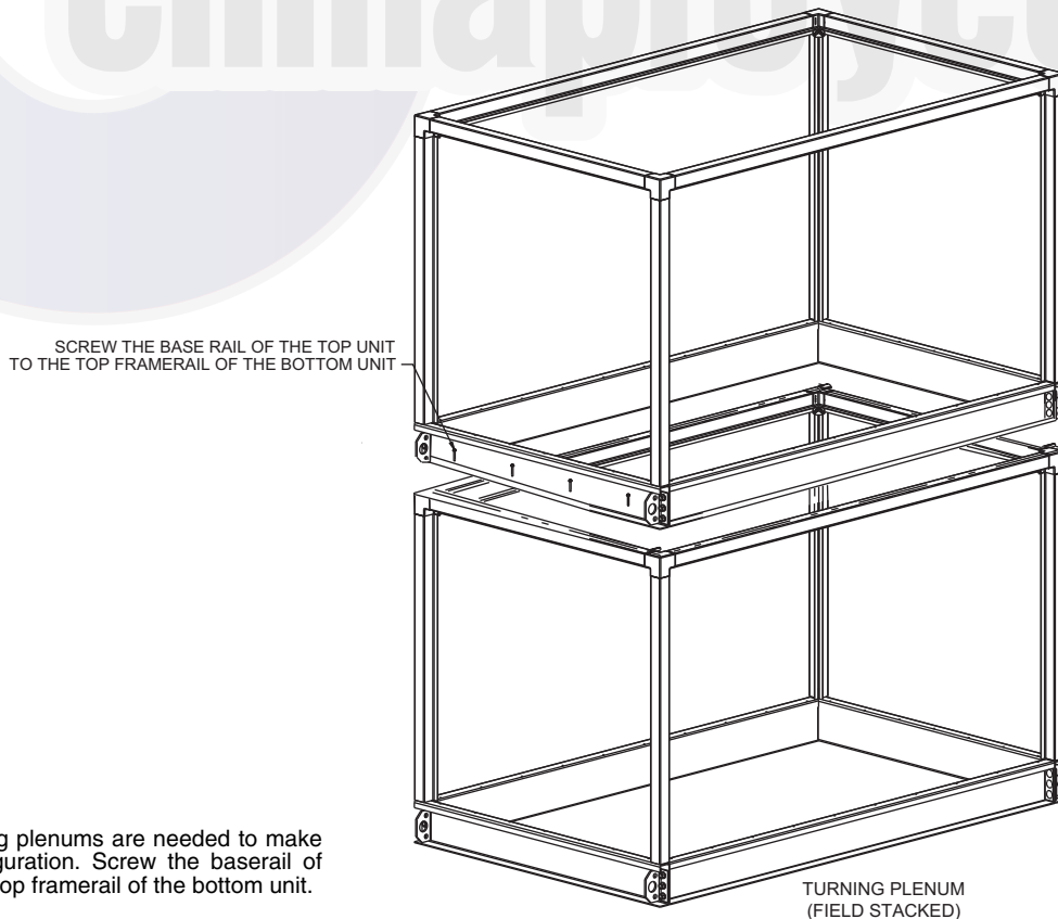
Fig. 43 — Stacked Turning Plenum
