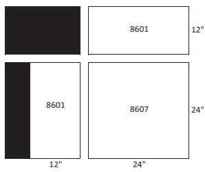
UNIT SIZE: 9T (1) 24" X 24" FILTER (2) 12" X 24" FILTERS
