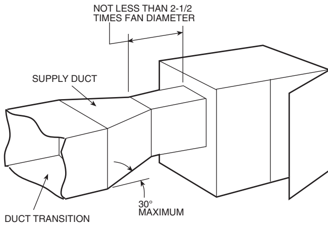
Fig. 34 — Duct Connections
