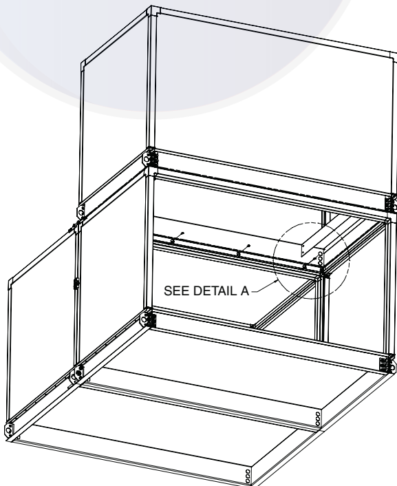
Fig. 27 — Attaching Split Sections — Stacked Units
