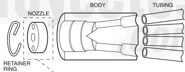
Fig. 97 — Distributor and Cap
