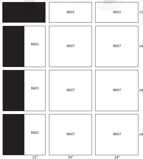
UNIT SIZE: 37T (6) 24" X 24" FILTERS (5) 12" X 24" FILTERS
