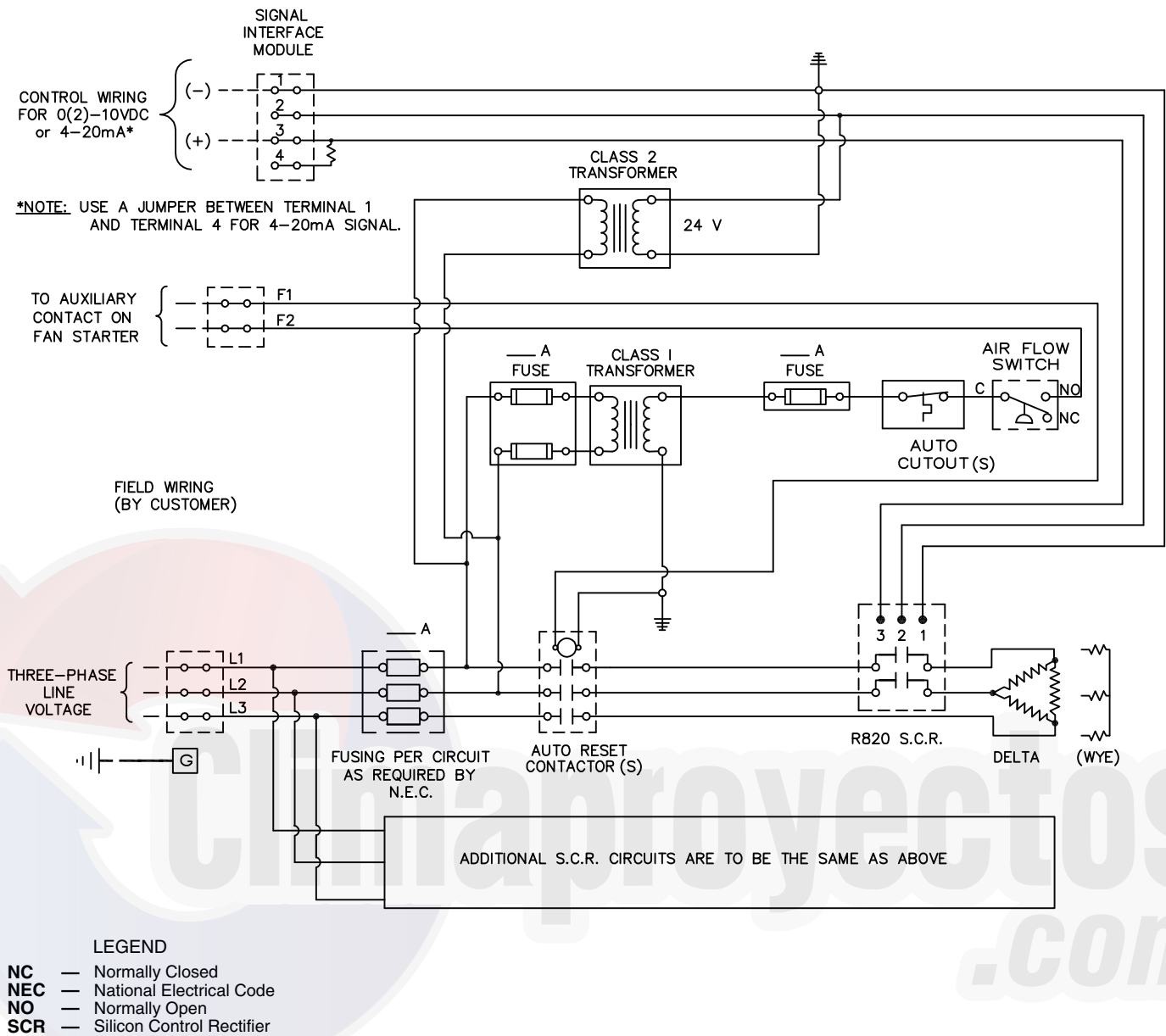
Fig. 130 — Full SCR Electric Heat Control
