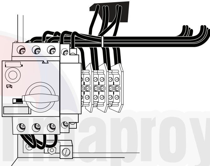
Fig. 121 — Connecting Shunt Trip Device to MMS
