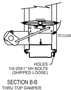
Fig. 36 — Face and Bypass Section Detail
