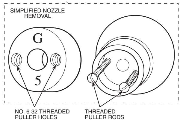
Fig. 98 — Nozzle Change-Out
