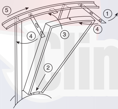
Fig. 166 — Segment Installation
