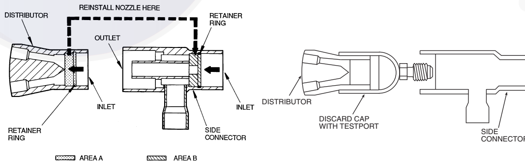
Fig. 101 — Distributor and Hot Gas Bypass Auxiliary Side Connector
