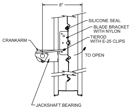
SECTION A-A THRU MIDDLE AND BOTTOM DAMPER
