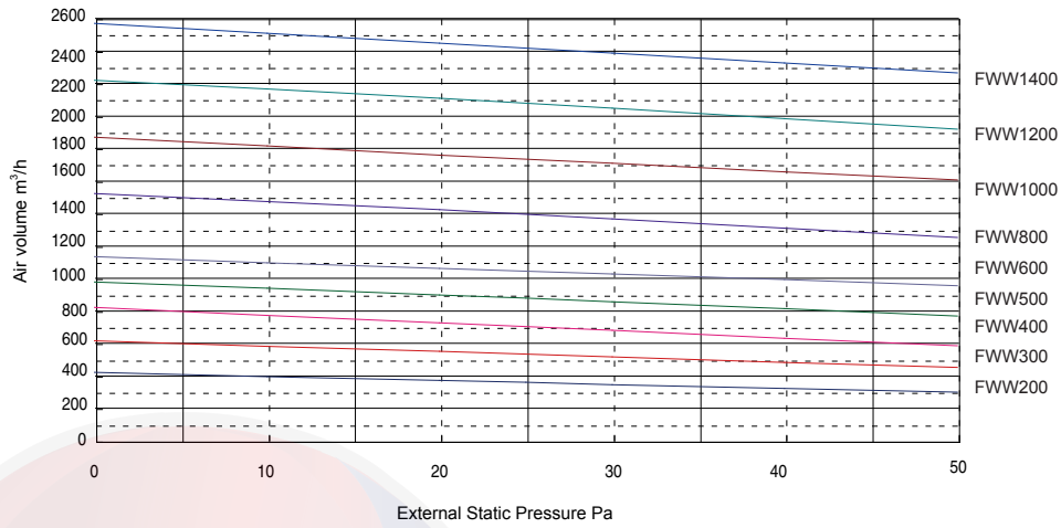
Outlet static pressure 30Pa H speed
