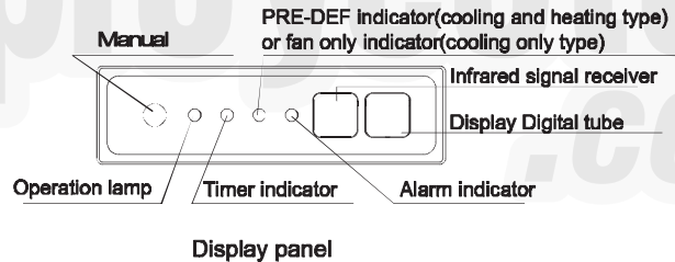
Fig. 6 — IR Receiver Display Panel
