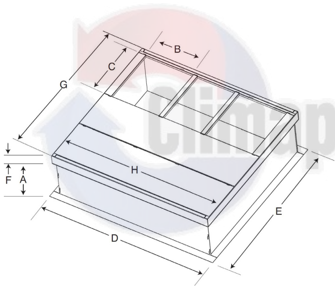
LARGE CURB
