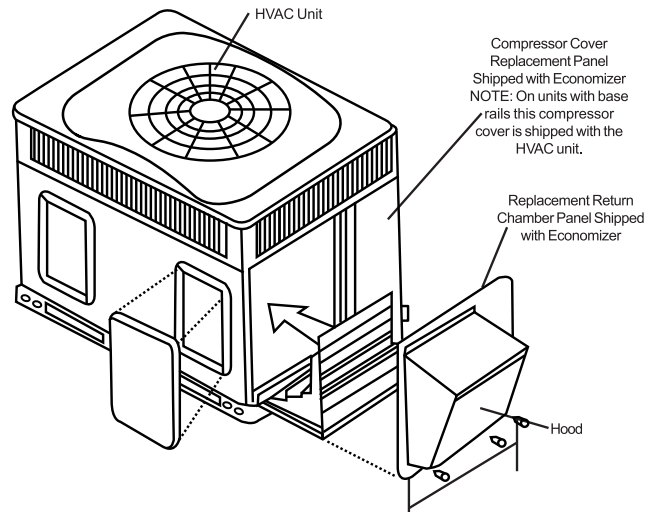
Vertical Economizer
